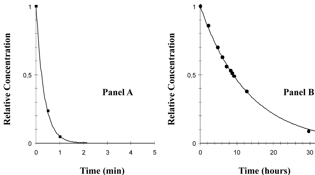
Figure 2. Relative concentration versus time curves for d 4 A (■, panel A) and 2',3'-dideoxy-2',3'-didehydro-3'-C-CF 3 adenosine ( 8 , ●, panel B) in Glycine/HCl buffer (pH 2) at 37 °C.
