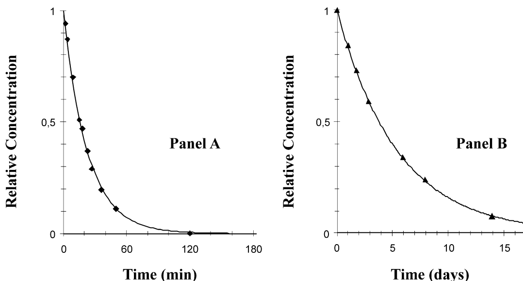
Figure 1. Relative concentration versus time curves for ddA (♦, panel A) and 2',3'-dideoxy-3'-C-CF 3 adenosine ( 6 , ▲, panel B) in Glycine/HCl buffer (pH 2) at 37 °C.
