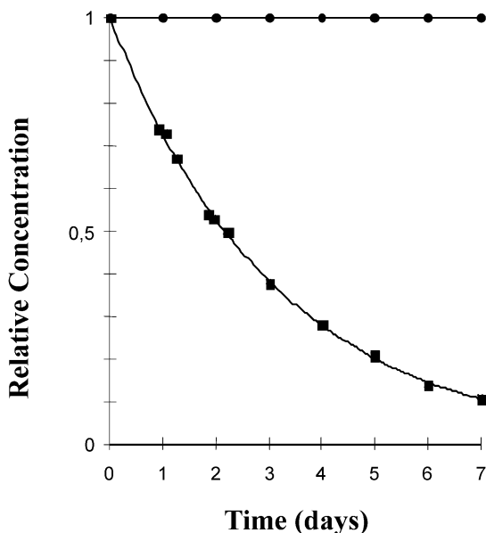
Figure 3. Relative concentration versus time curves for d 4 A (■) and 2',3'-dideoxy-2',3'-didehydro-3'-C-CF 3 adenosine ( 8 , ●) in phosphate buffer (pH 7.2) at 37 °C.
