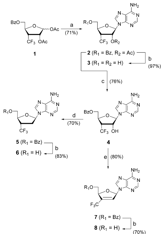
Scheme 1. (a) Adenine, \text{SnCl}_4 , \text{CH}_3\text{CN} , rt; (b) \text{NH}_3/\text{MeOH} , rt; (c) \text{H}_2\text{NNH}_2 , \text{AcOH} , pyridine, rt; (d) (i) DMAP, \text{C}_6\text{H}_5\text{O}(\text{S})\text{Cl} , \text{CH}_3\text{CN} , rt; (ii) (\text{Me}_3\text{Si})_3\text{SiH} , AIBN, toluene, reflux; (e) (i) \text{MsCl} , pyridine, rt; (ii) TBAF, THF, 50^\circ\text{C} .
