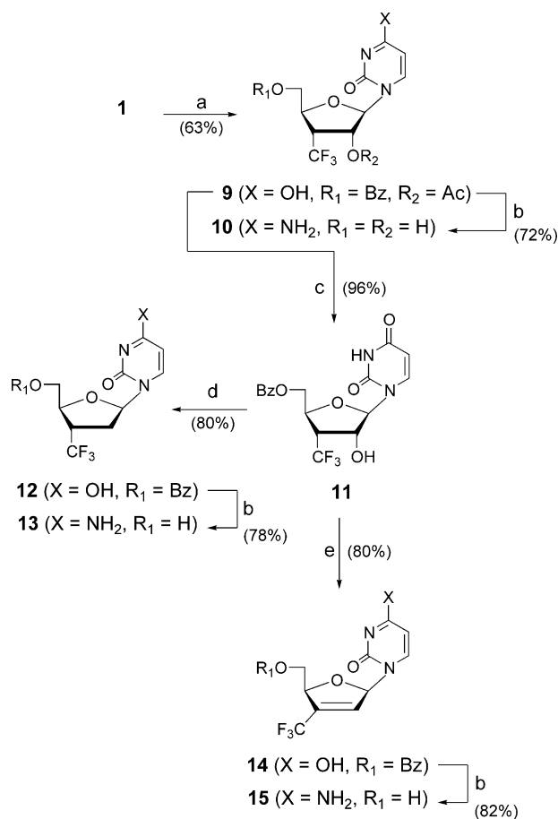
Scheme 2. (a) Silylated uracil, TMSOTf, 1,2-dichloroethane, rt; (b) (i) 1-methylpyrrolidine, CH 3 CN, (CF 3 CO) 2 O, 0 °C; (ii) 4-nitrophenol, 0 °C; (iii) coned aq NH 3 /dioxane, 55 °C; (iv) NH 3 /MeOH, rt; (c) H 2 NNH 2 , AcOH, pyridine, rt; (d) (i) pyridine, C 6 H 5 O(S)Cl, CH 2 Cl 2 , rt; (ii) (Me 3 Si) 3 SiH, AIBN, toluene, reflux; (e) (i) MsCl, pyridine, rt; (ii) TBAF, THF, 50 °C.
